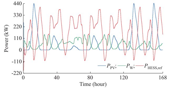
Fig. 5. Output power of PV array and WECS and output power reference of HESS.
