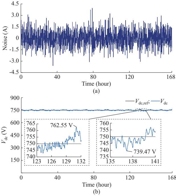
Fig. 10. DC bus voltage performance with a white noise disturbance under load condition in Fig. 4. (a) Injected Gaussian white noise signal (zero-mean, unit-variance). (b) Resulting bus voltage waveform.
