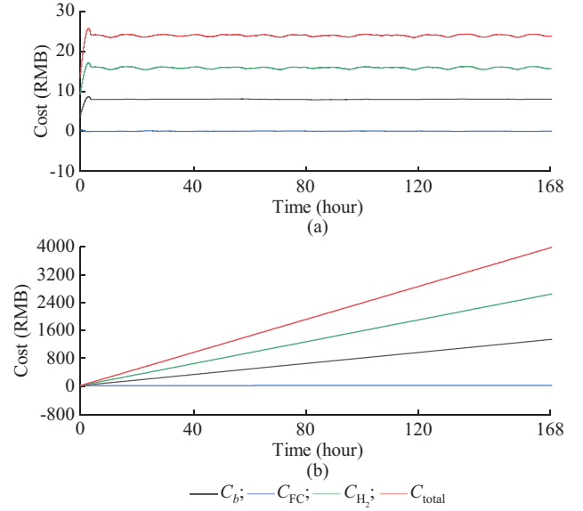
Fig. 8. Variations in hydrogen consumption cost, aging cost of PEMFC, aging cost of LIB, and total consumption cost over 168-hour operation period under EEMS. (a) Real-time costs. (b) Cumulative costs.
