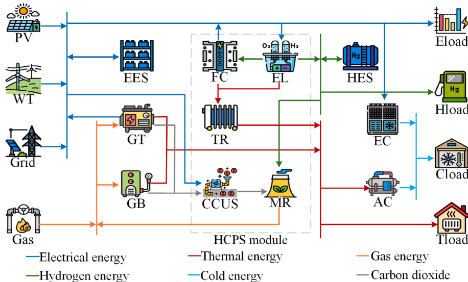
Fig. 1. Structure diagram of the IES.
