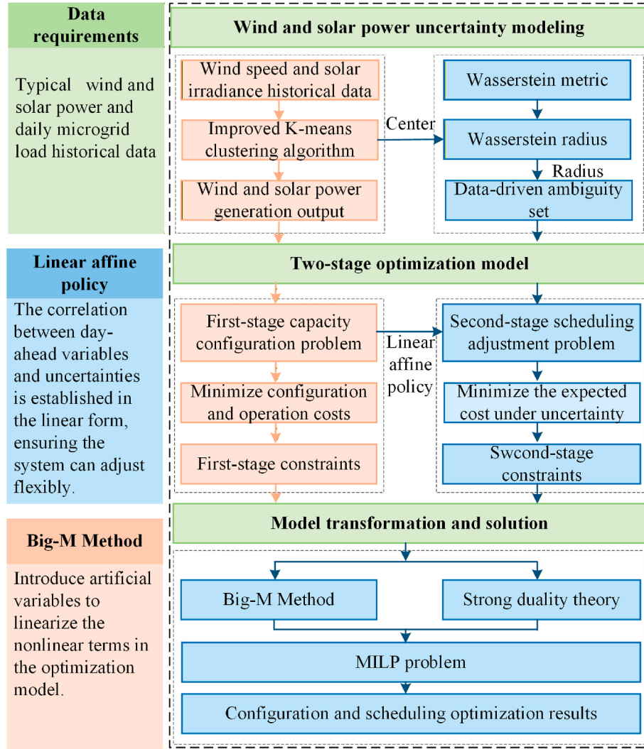
Fig. 3. The framework of modeling and solving procedure.
