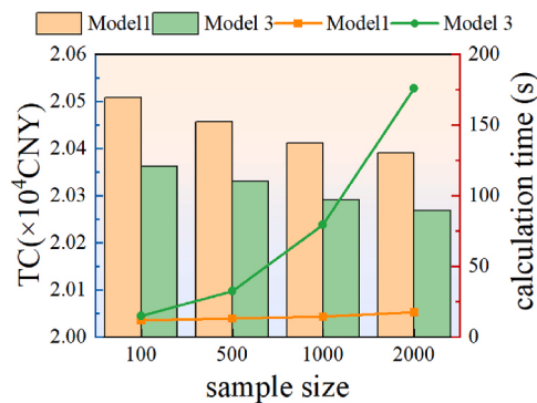
Fig. 13. System optimization results and computation time under different sample sizes.
