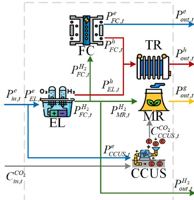
Fig. 2. The synergistic HCPs module.
