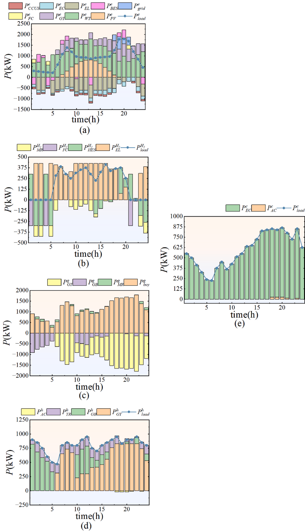
Fig. 9. Optimal dispatch results for (a) electrical power, (b) hydrogen, (c) natural gas, (d) thermal energy, (e) cooling energy.
