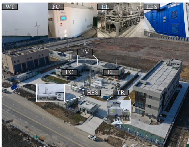
Fig. 4. Actual IES case from a demonstration project in the coastal area of Zhejiang, China.
