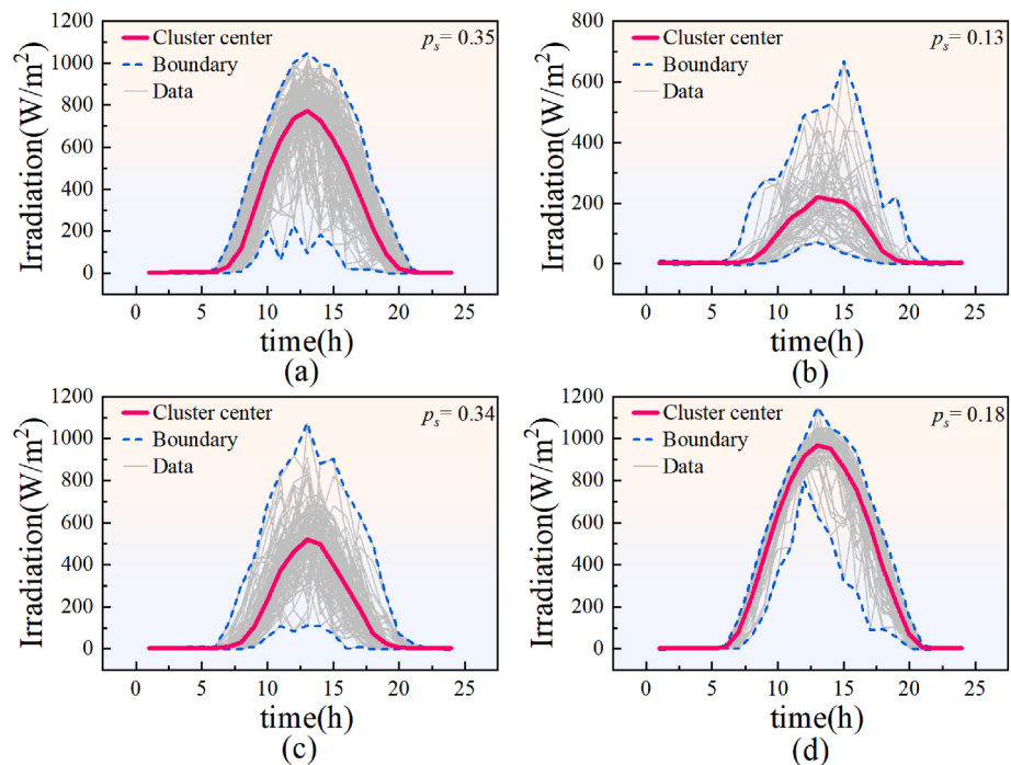
Fig. 6. Solar irradiance scenario construction and corresponding probabilities.
