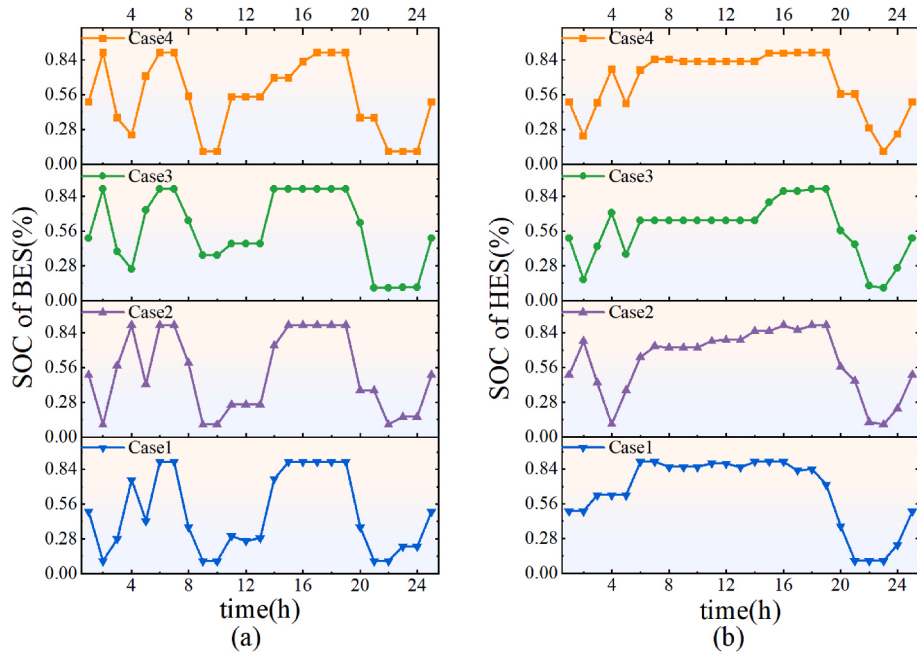
Fig. 10. Hybrid hydrogen-electric energy storage dispatch optimization results, (a) SOC of BES, (b) SOC of HES.
