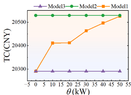
Fig. 12. Influence of parameter \theta on system optimization costs.
