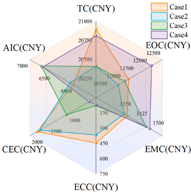
Fig. 8. System configuration optimization results under different cases.
