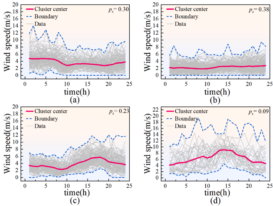
Fig. 5. Wind speed scenario construction and corresponding probabilities.
