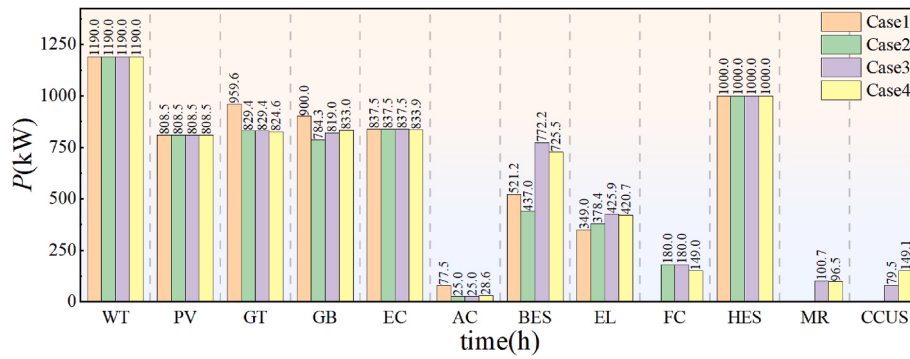
Fig. 7. The IES capacity configuration results.
